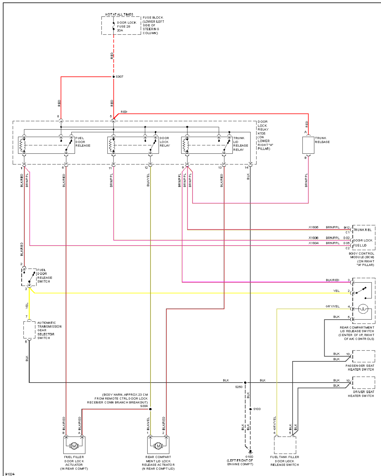
Fig. 44: Trunk & Fuel Door Release Circuit
