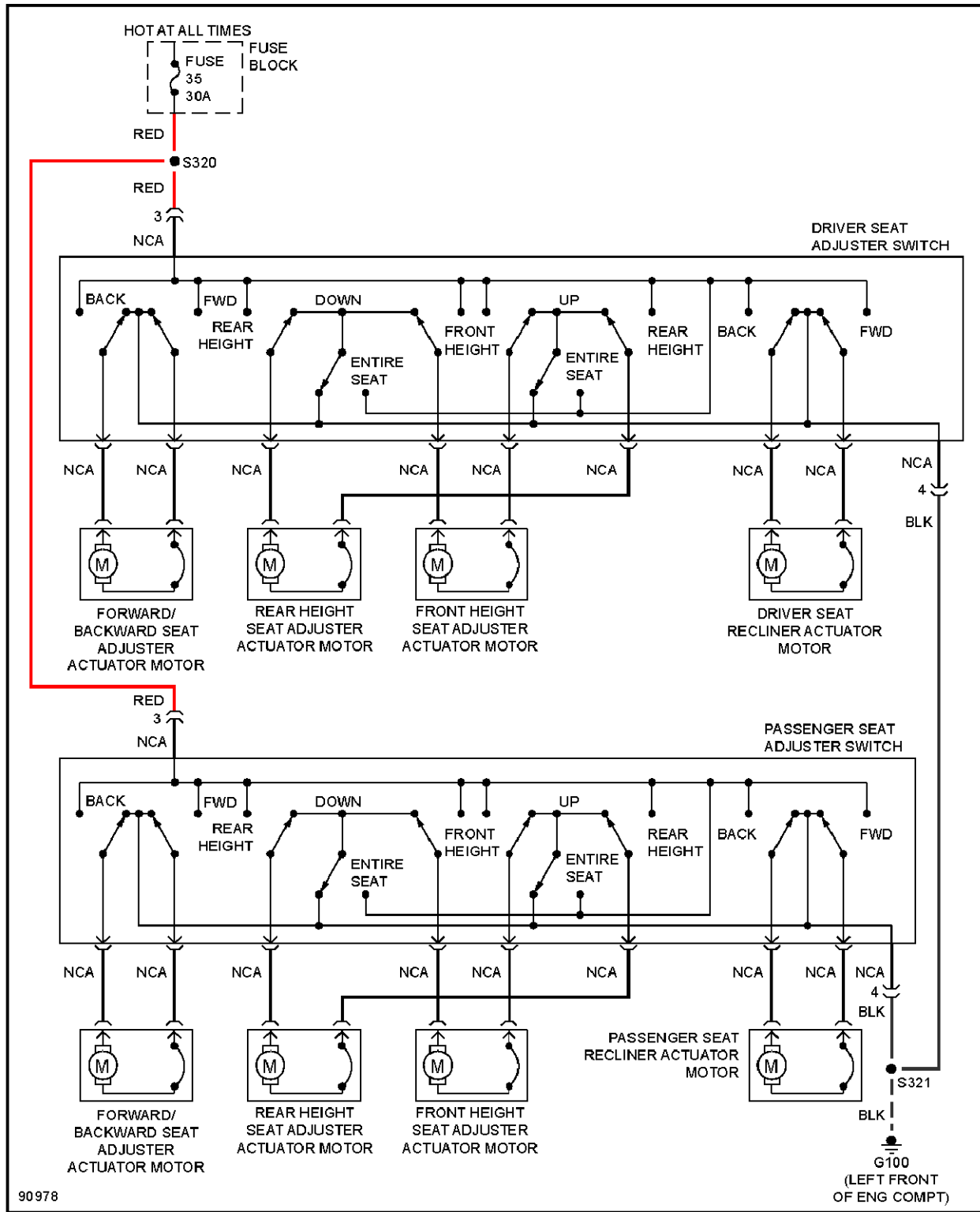
Fig. 31: 6-Way & Recliner Power Seat Circuit
