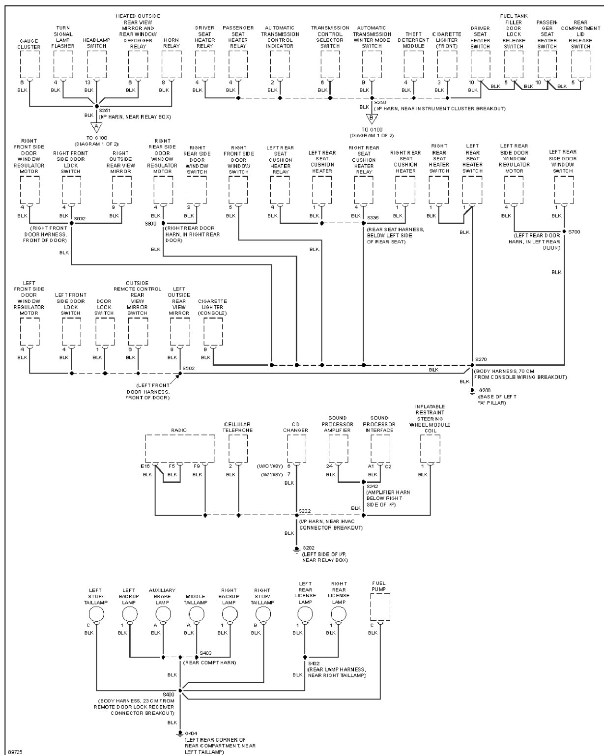
Fig. 18: Ground Distribution Circuit (2 of 2)
