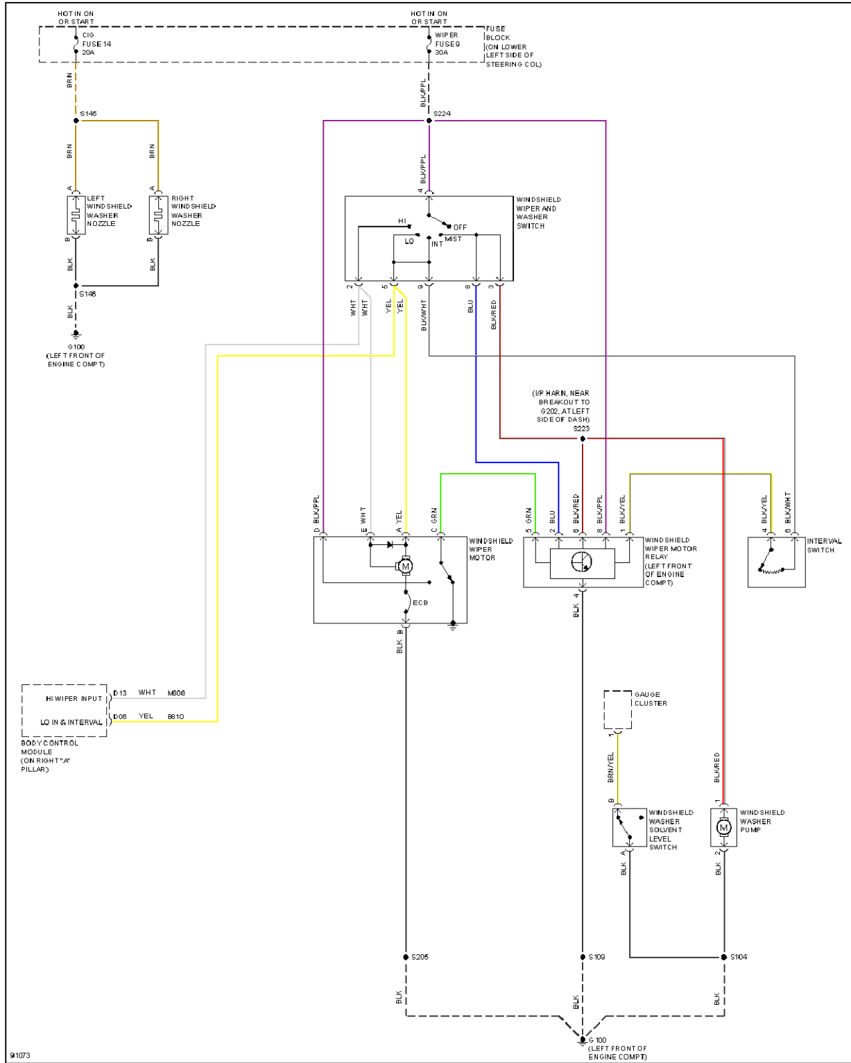
Fig. 46: Wiper/Washer Circuit
