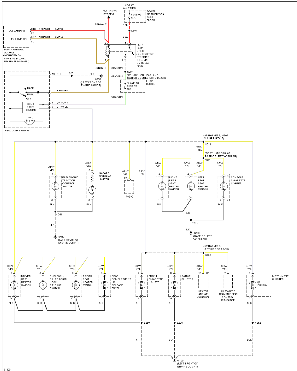
Fig. 23: Instrument Illumination Circuit
