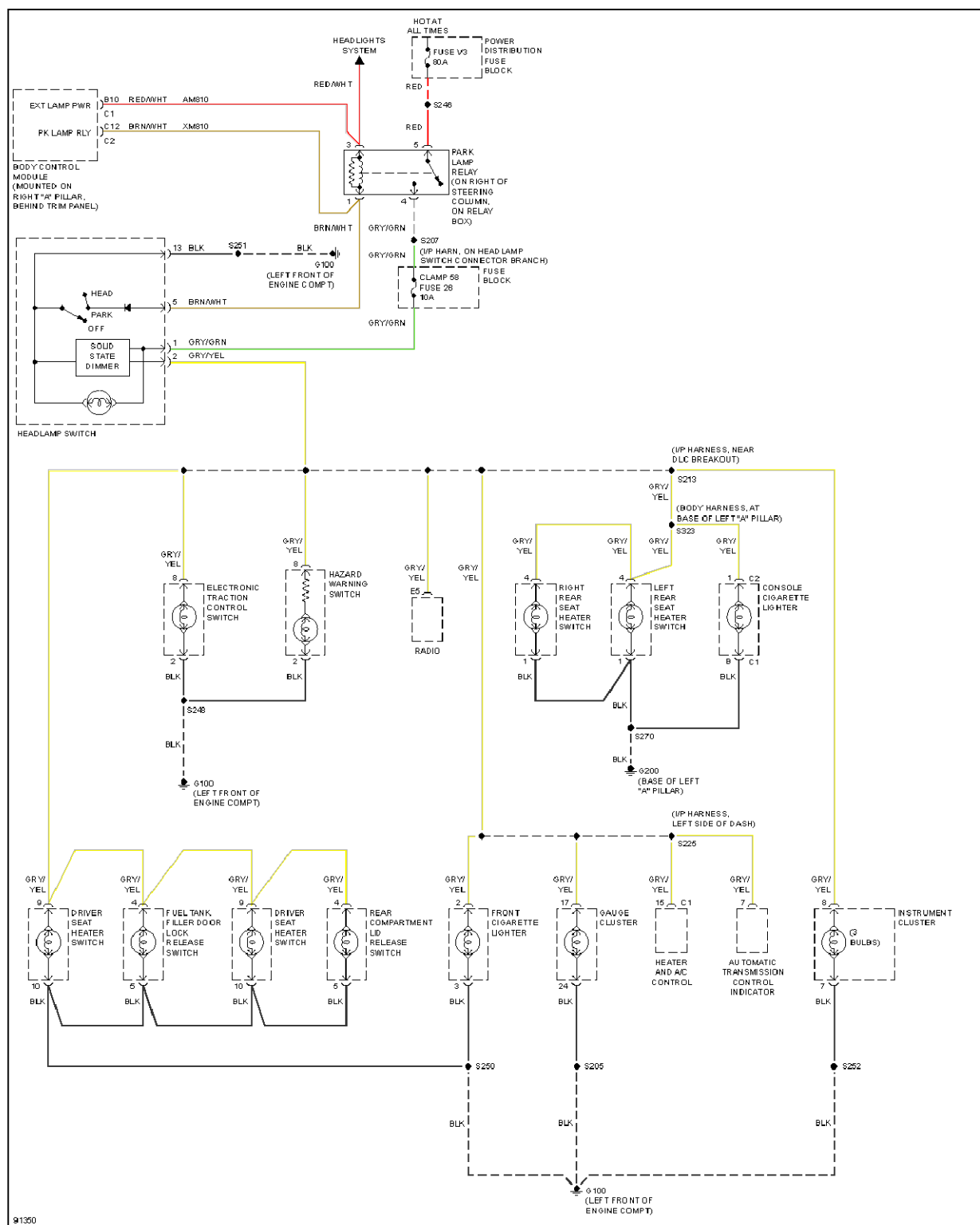
Fig. 24: Instrument Illumination Circuit
