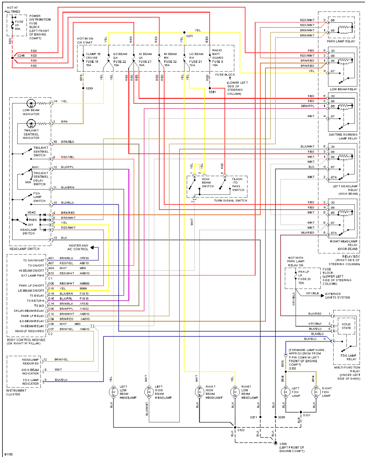
Fig. 20: Headlamps/Fog Lamps Circuit
