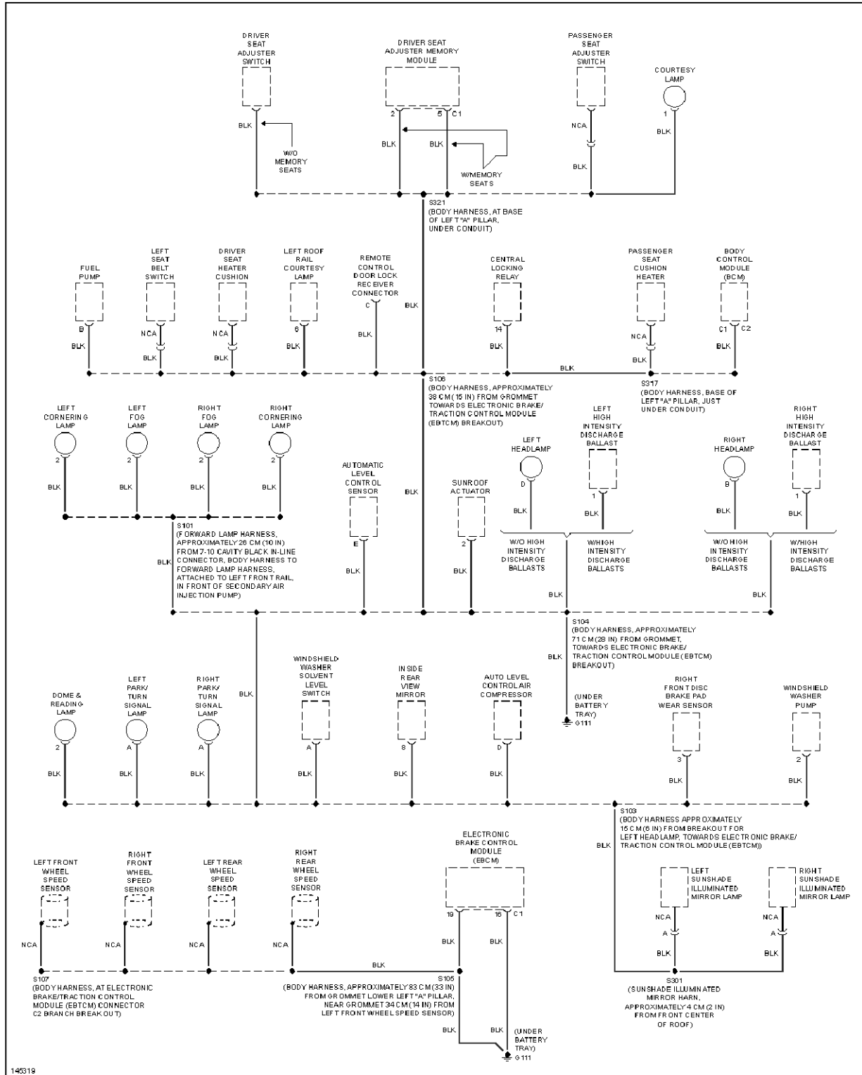
Fig. 19: Ground Distribution Circuit (2 of 3)
