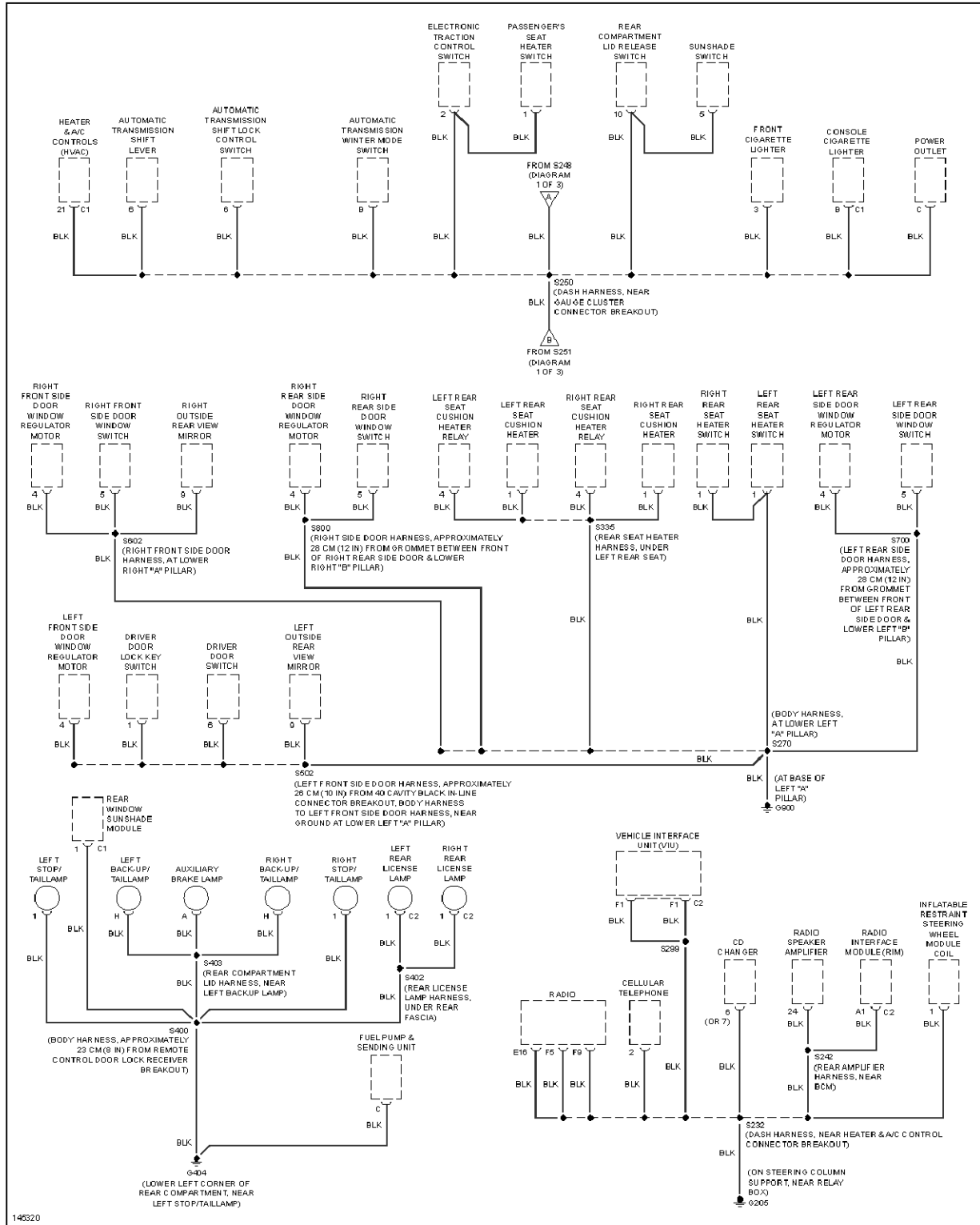
Fig. 20: Ground Distribution Circuit (3 of 3)
