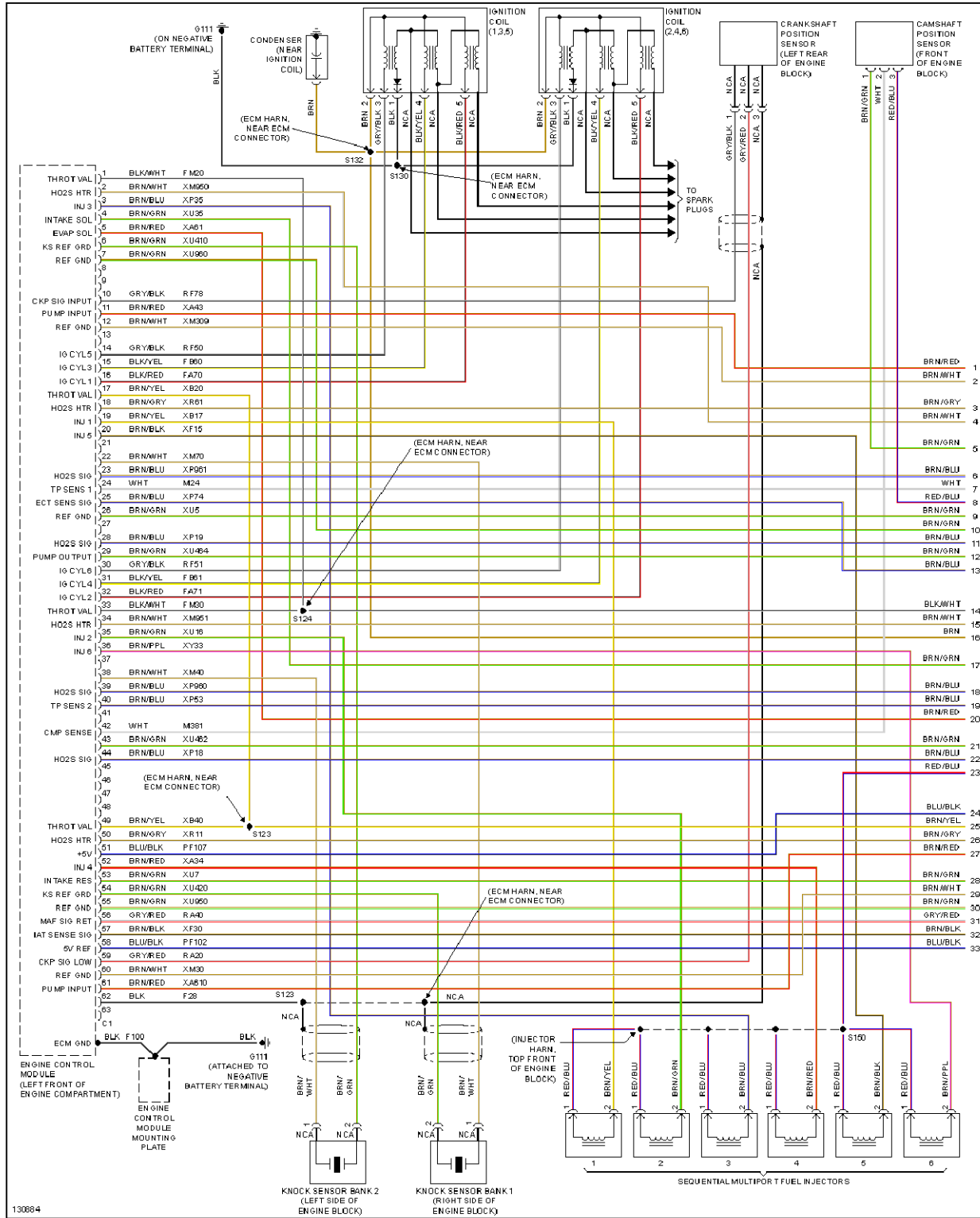
Fig. 13: 3.0L VIN R, Engine Performance Circuits (1 of 3)
