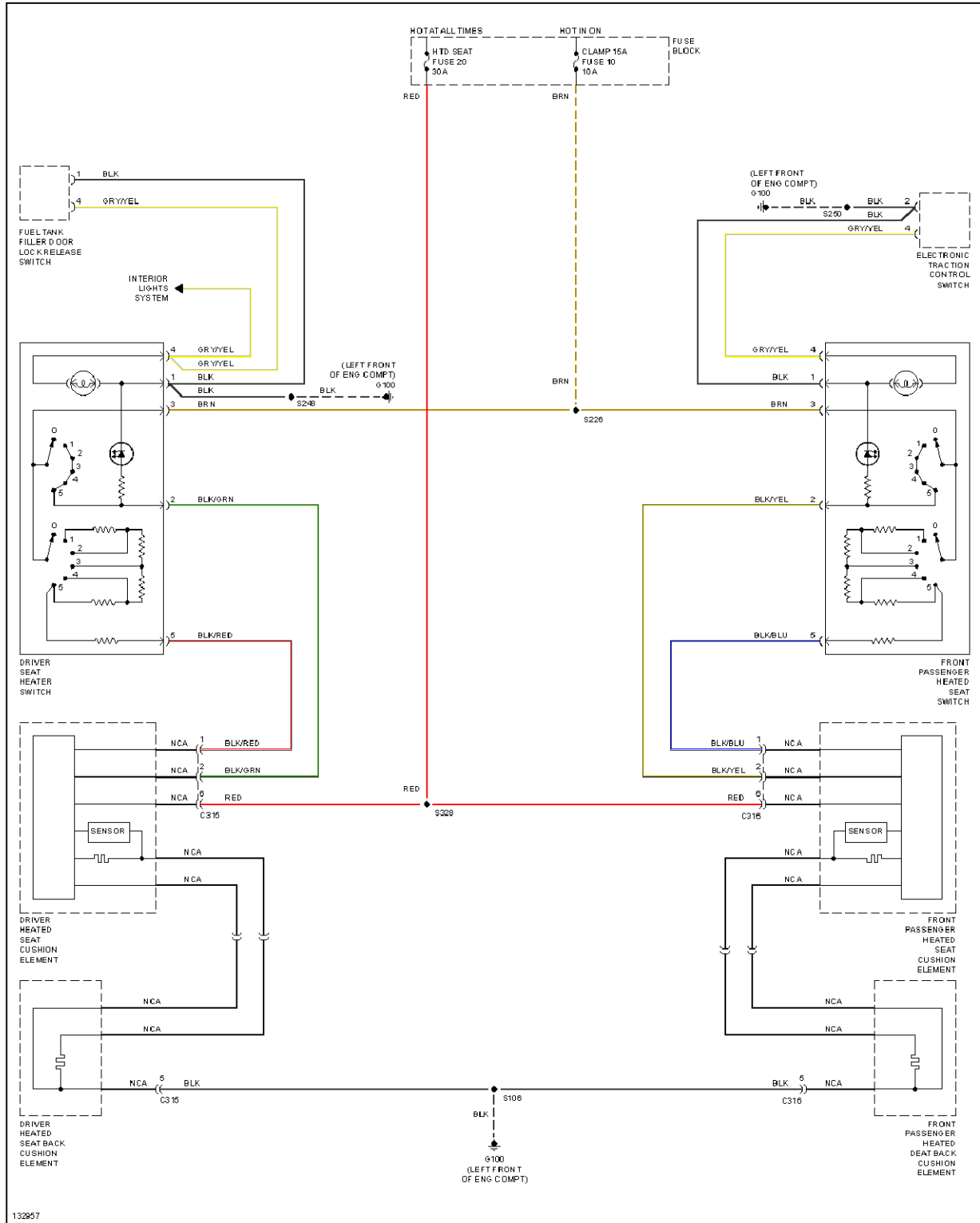
Fig. 35: Front Seat Heater Circuit
