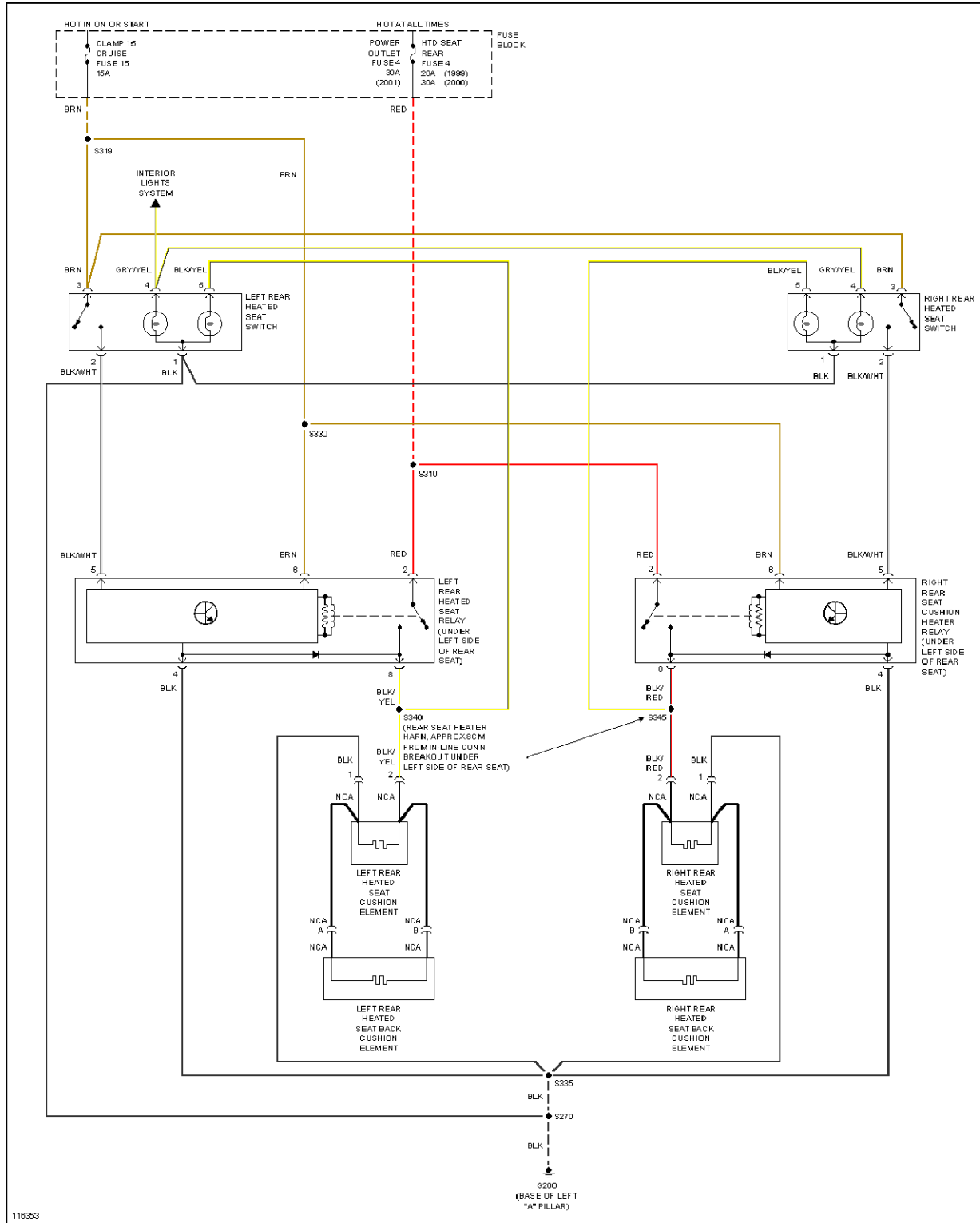
Fig. 36: Rear Seat Heater Circuit
