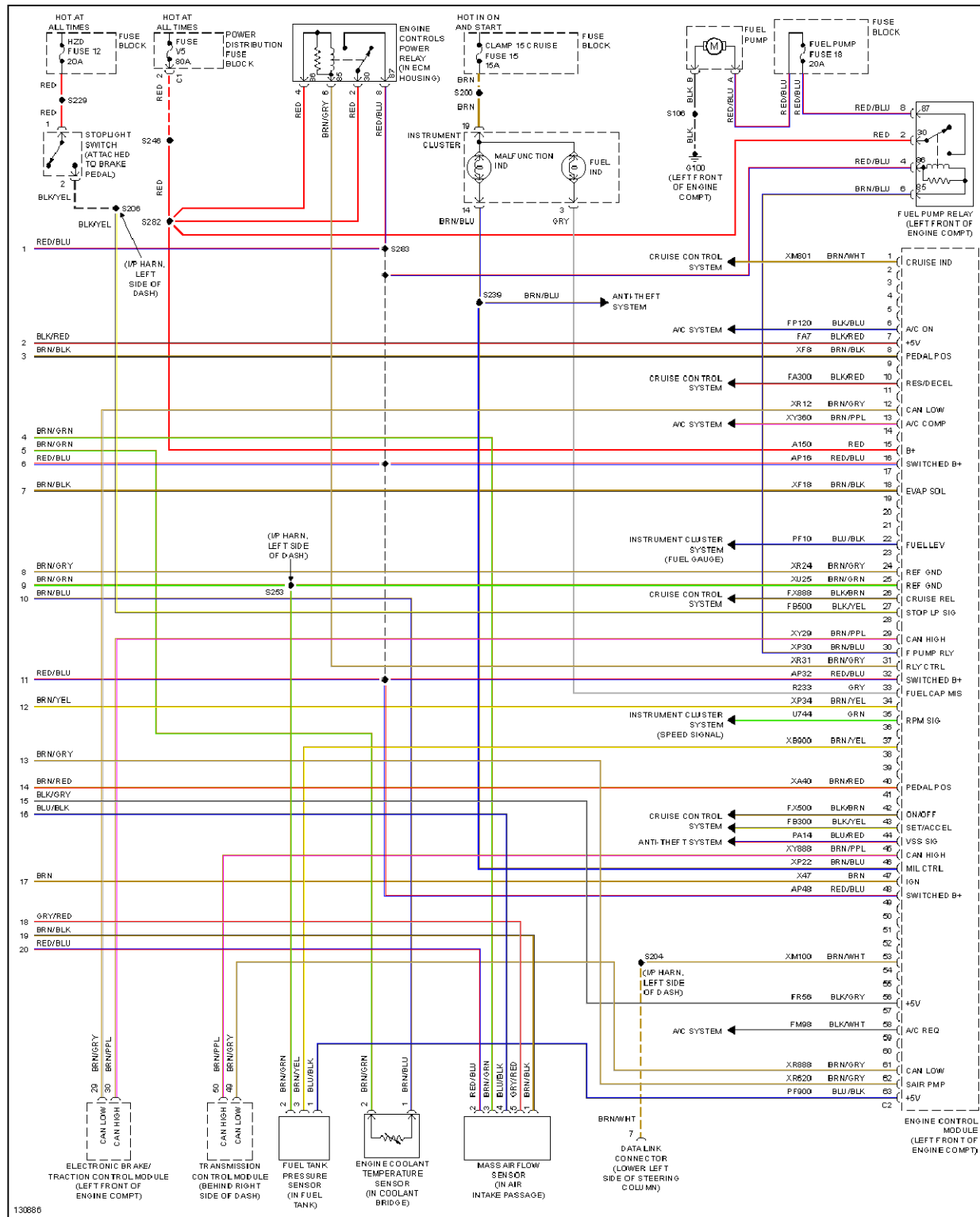
Fig. 15: 3.0L VIN R, Engine Performance Circuits (3 of 3)
