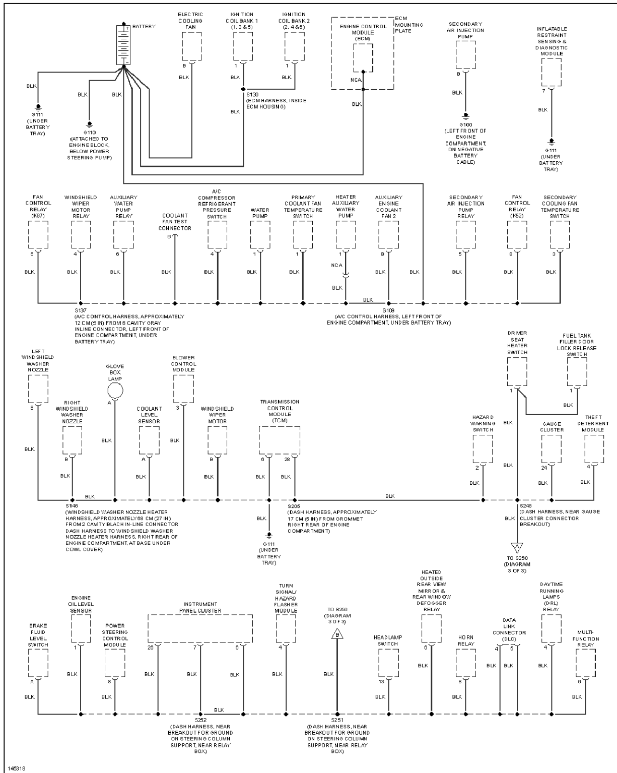
Fig. 18: Ground Distribution Circuit (1 of 3)
