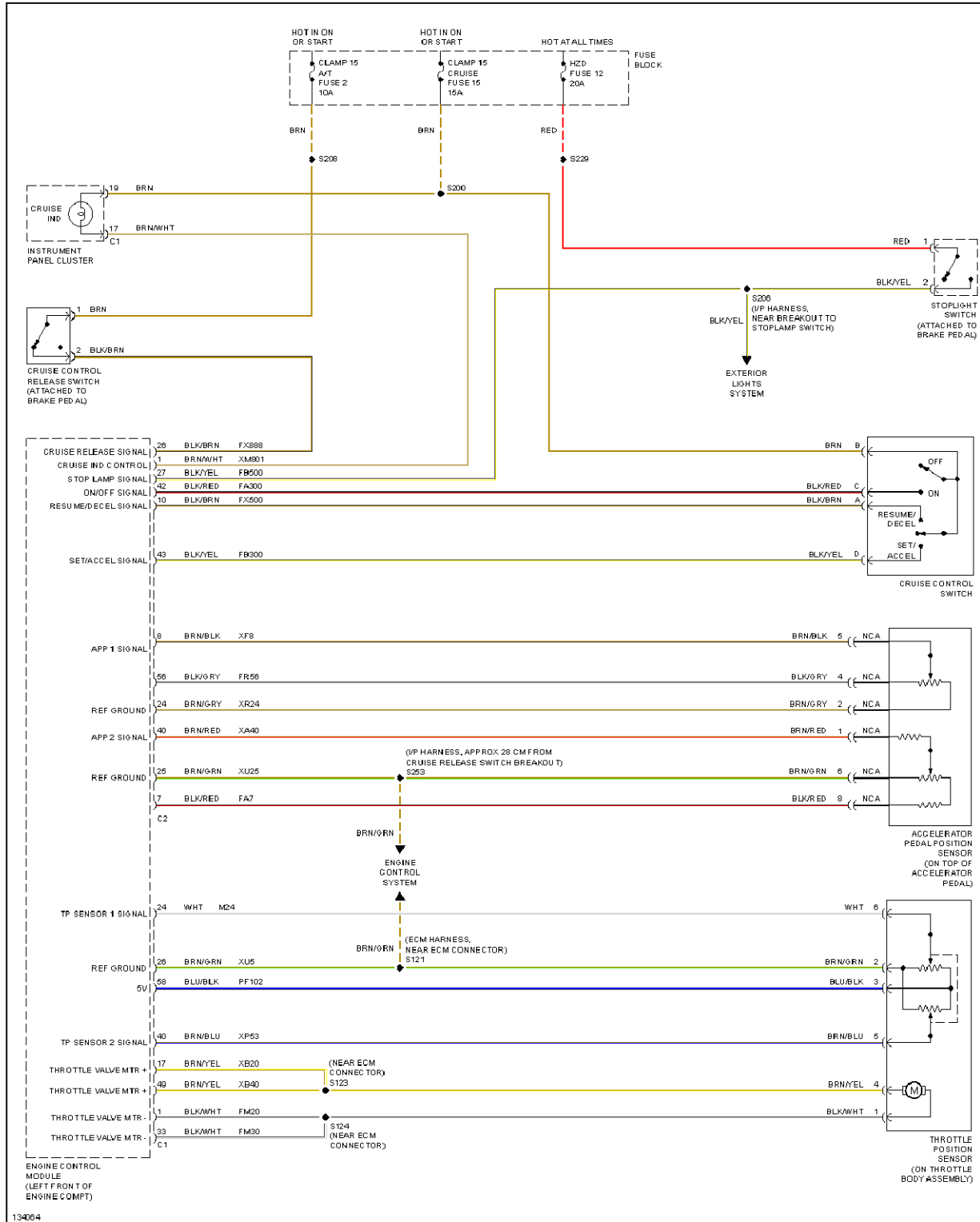
Fig. 9: Cruise Control Circuit
