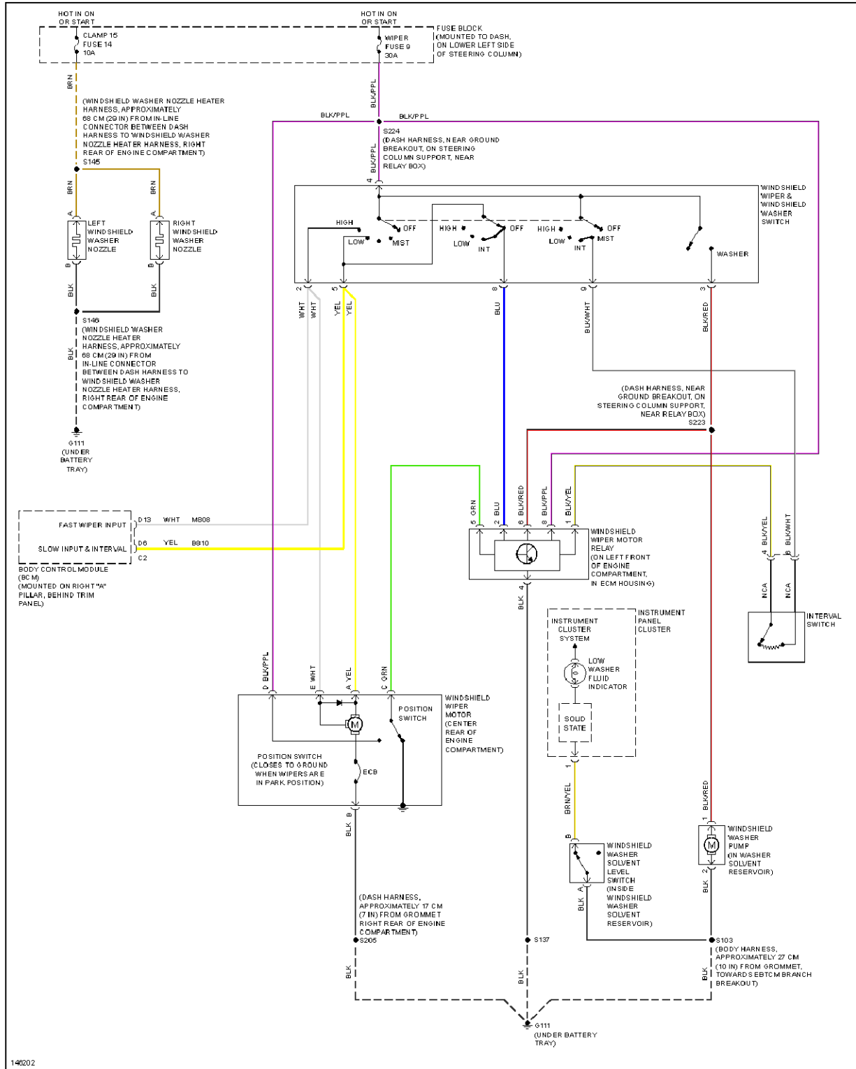
Fig. 49: Wiper/Washer Circuit
