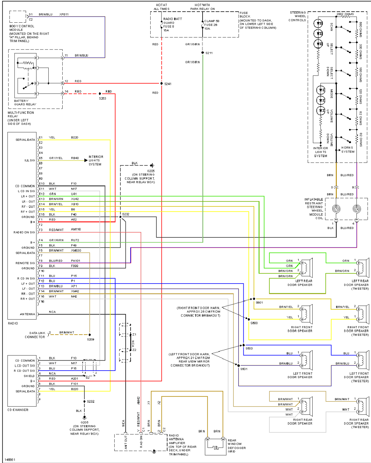
Fig. 39: Radio Circuits, Base Radio
