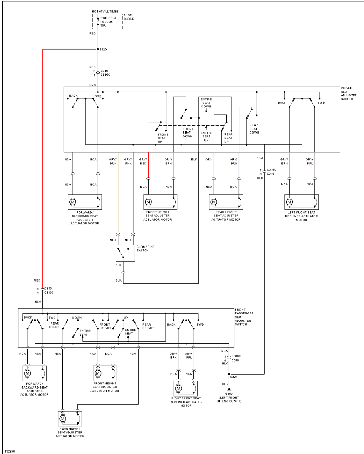
Fig. 34: 6-Way & Recliner Power Seat Circuit
