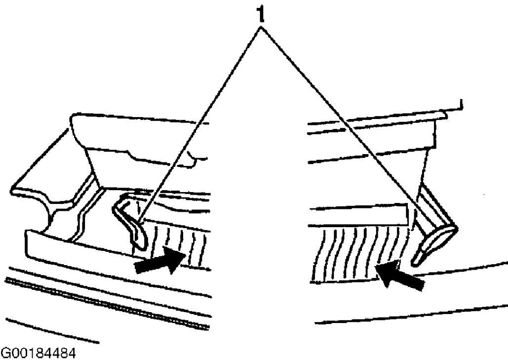
Fig. 2: Releasing Passenger Compartment Air (Pollen) Filter Courtesy of GENERAL MOTORS CORP.
